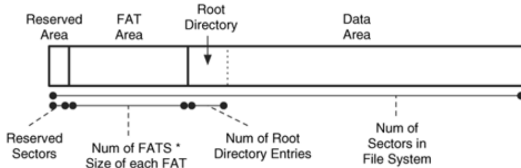
FAT12/16
